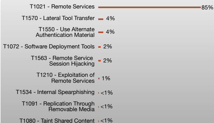
Figure 14. Relative prevalence of techniques observed in association with the lateral movement tactic.
