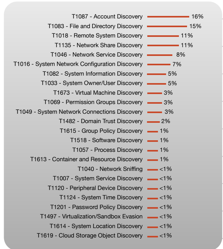
Figure 8. Relative prevalence of techniques observed in association with the discovery tactic.
