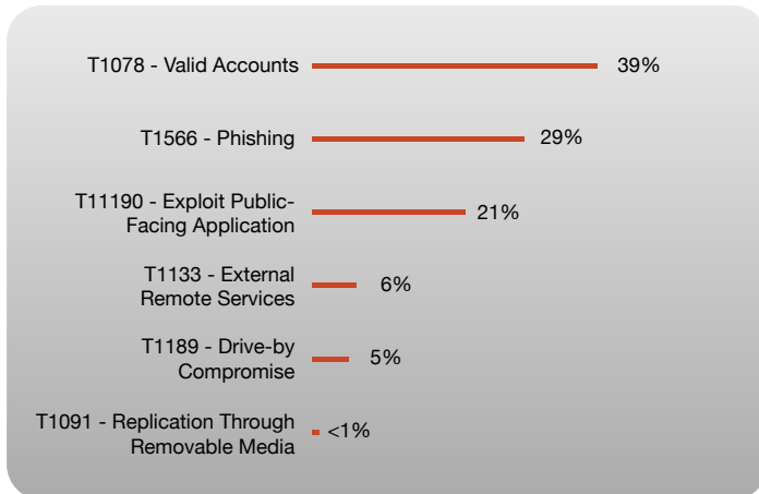
Figure 7. Relative prevalence of techniques observed in association with the initial access tactic.
