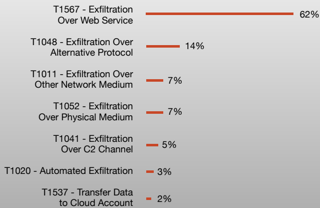
Figure 17. Relative prevalence of techniques observed in association with the exfiltration tactic.
