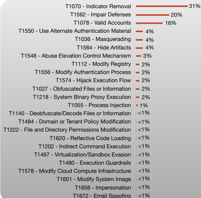
Figure 12. Relative prevalence of techniques observed in association with the defense evasion tactic.
