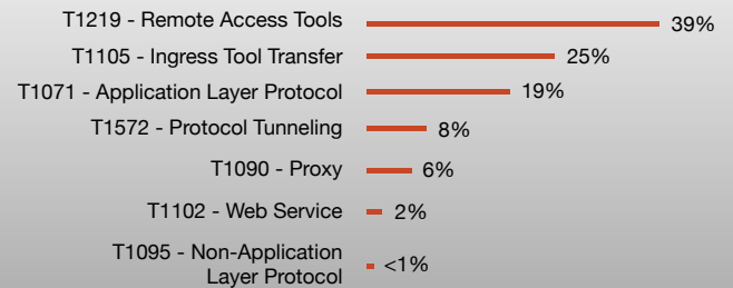
Figure 16. Relative prevalence of techniques observed in association with the command and control tactic.
