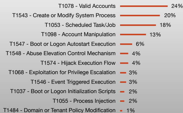
Figure 11. Relative prevalence of techniques observed in association with the privilege escalation tactic.
