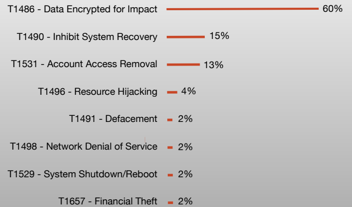
Figure 18. Relative prevalence of techniques observed in association with the impact tactic.
