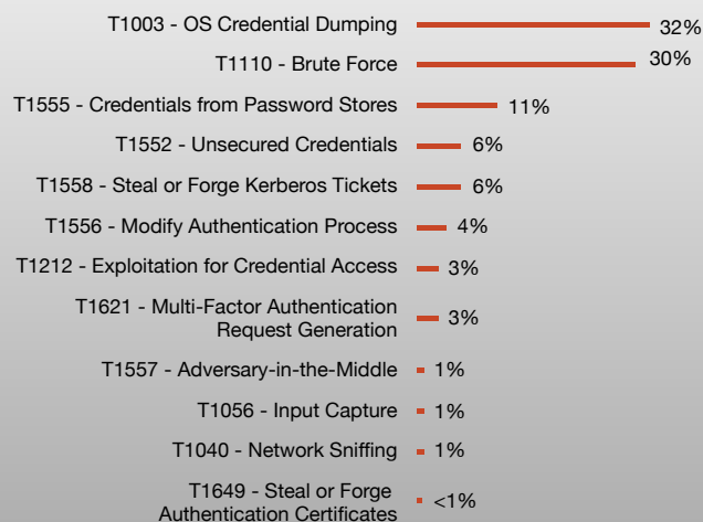
Figure 13. Relative prevalence of techniques observed in association with the credential access tactic.
